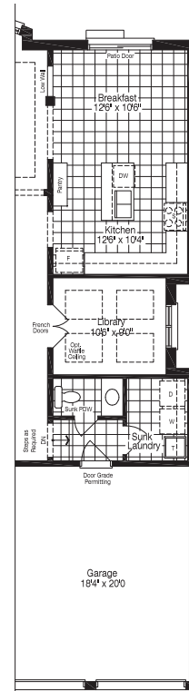
GROUND FLOOR ELEV-A PARTIAL PLAN OPTION GROUND FLOOR LAUNDRY
