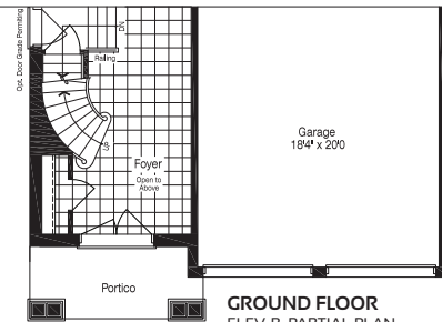
GROUND FLOOR ELEV-A
